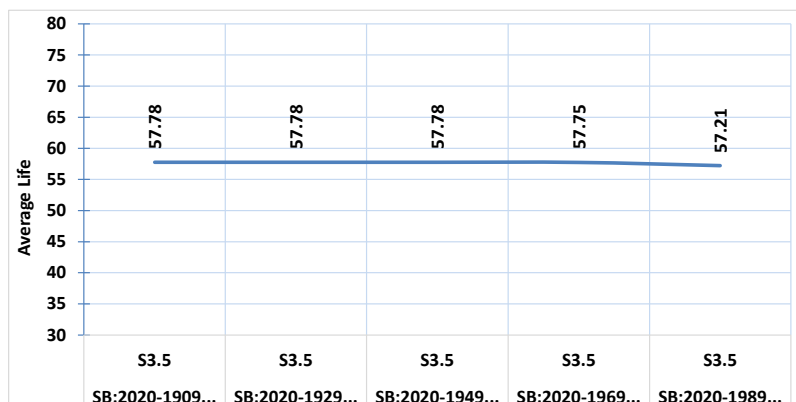
Figure 32. Worm Chart for Steam Turbines (Non-CC)
